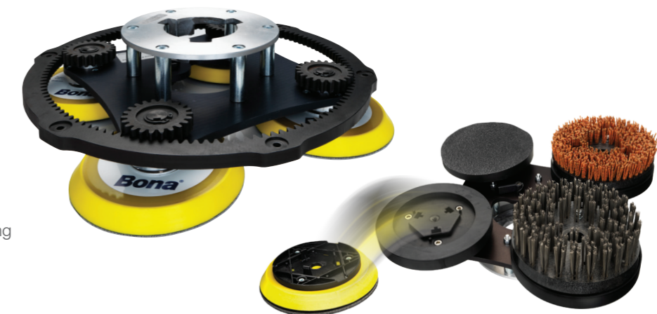
Click-on 'Connect' system for mounting Brushes and Sanding Discs
